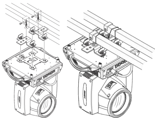
Figure 2 Flip-up luminaire diagram
