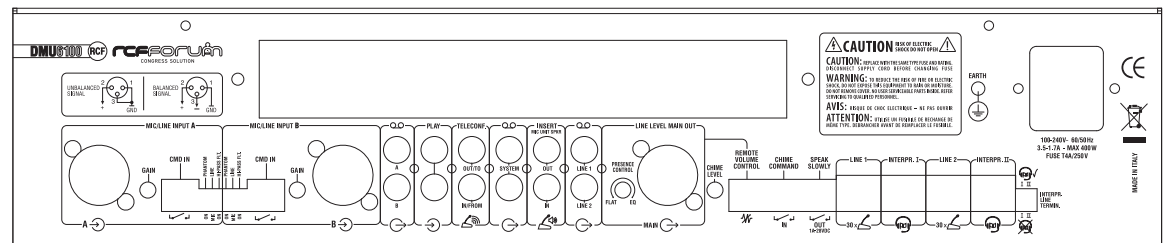
Rear panel
